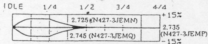
(3) Jet Needle (Straight Section)
