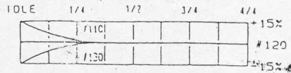
(7) Pilot Screw
