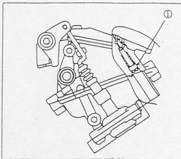
1. Pilot Screw
