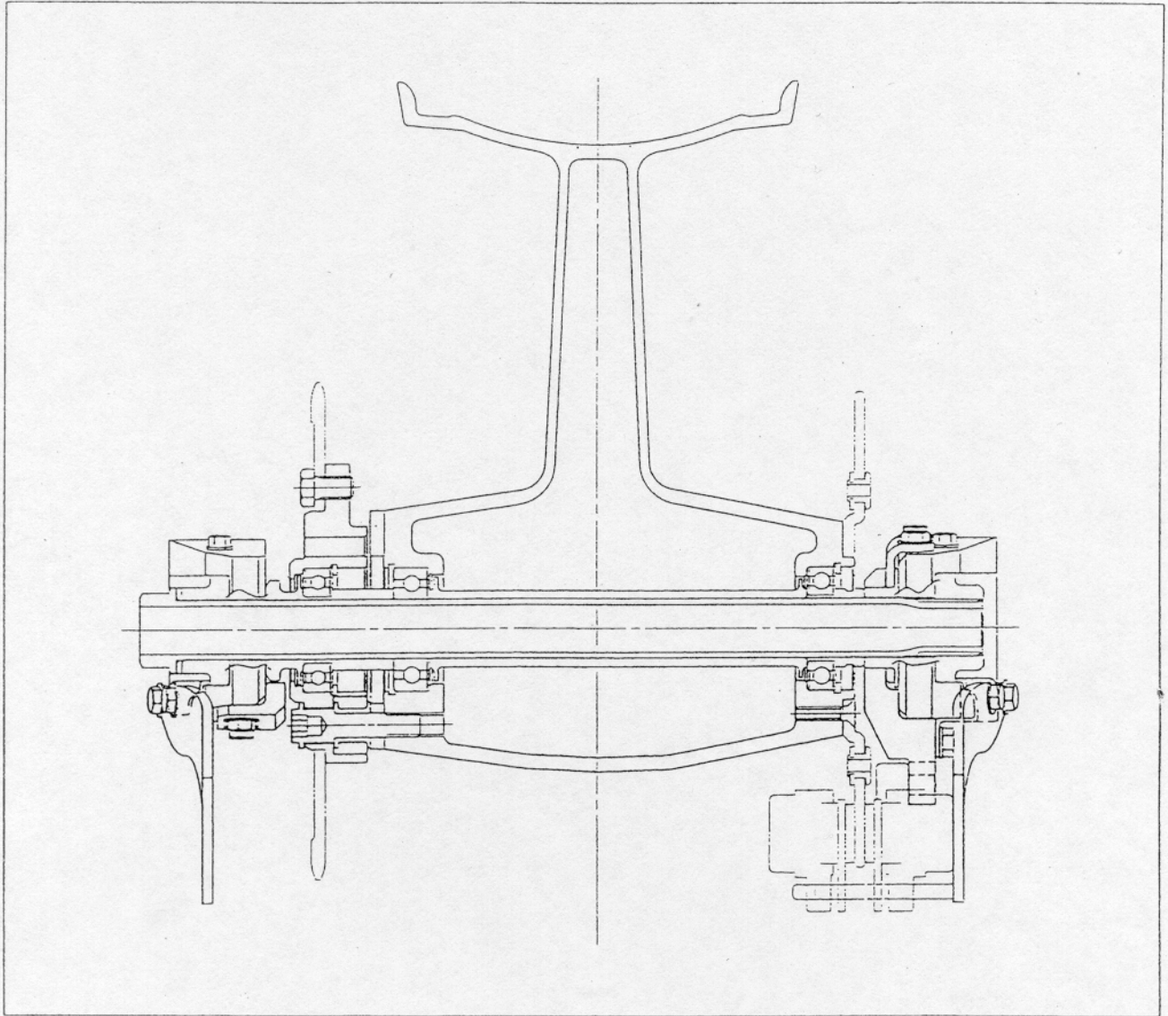
Section View
